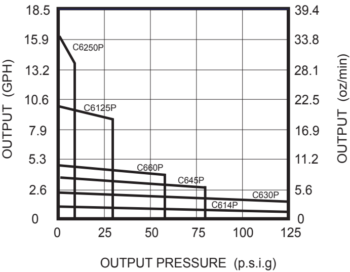
Maximum Output vs. Pressure Curve
